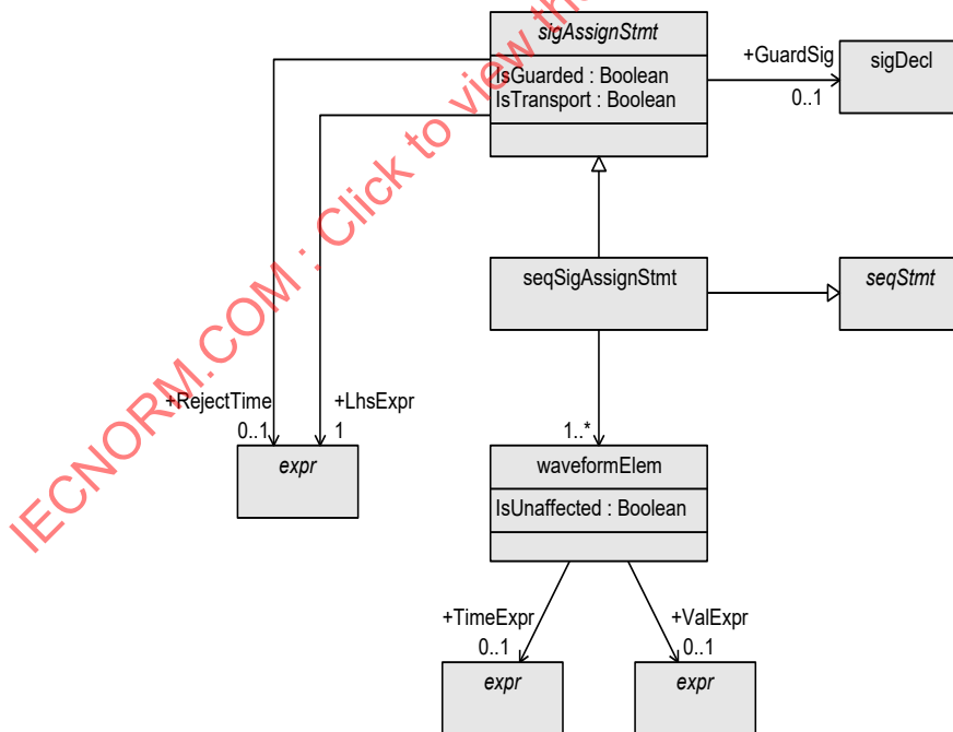
Figure 41—SeqSigAssignStmt class diagram
