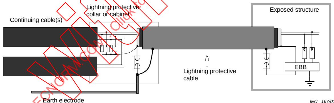
Figure 7a – Unshielded cable
