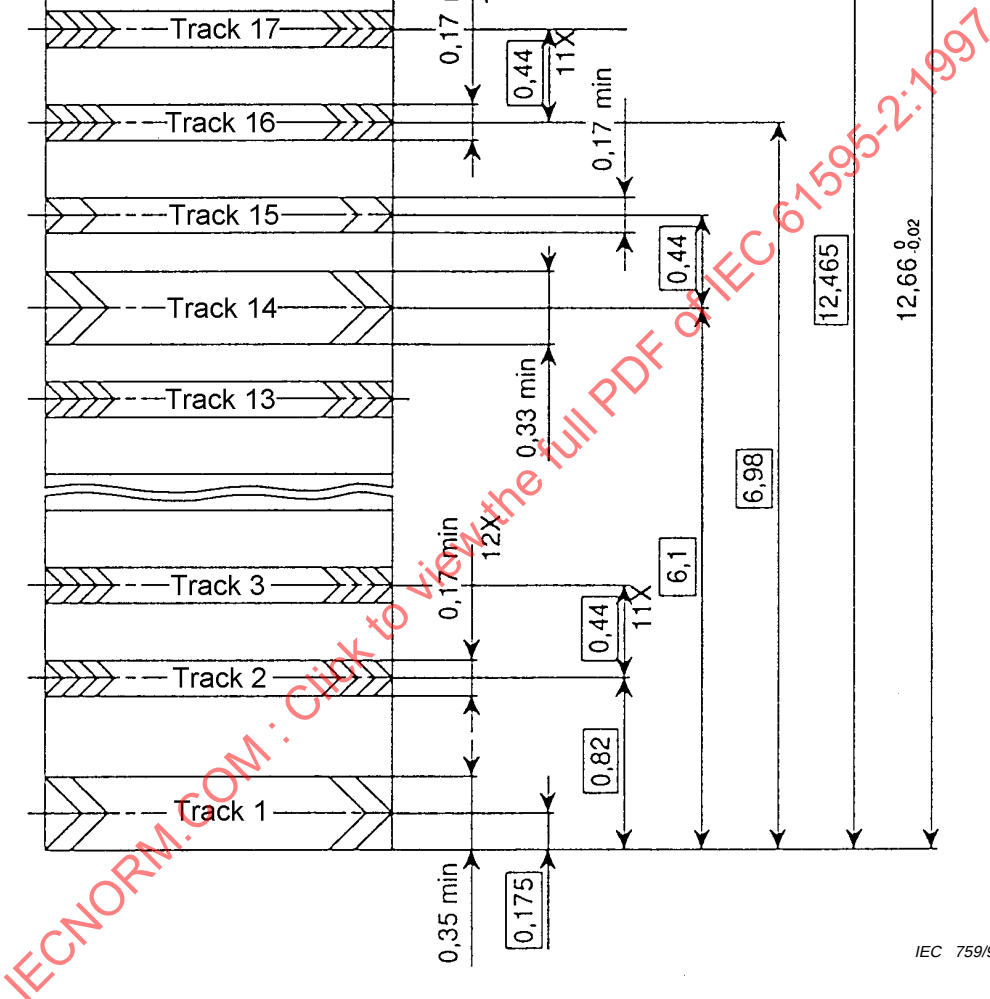
Figure 4 – Track pattern for DATR on magnetic tape (28 tracks with 12,7 mm tape width)
