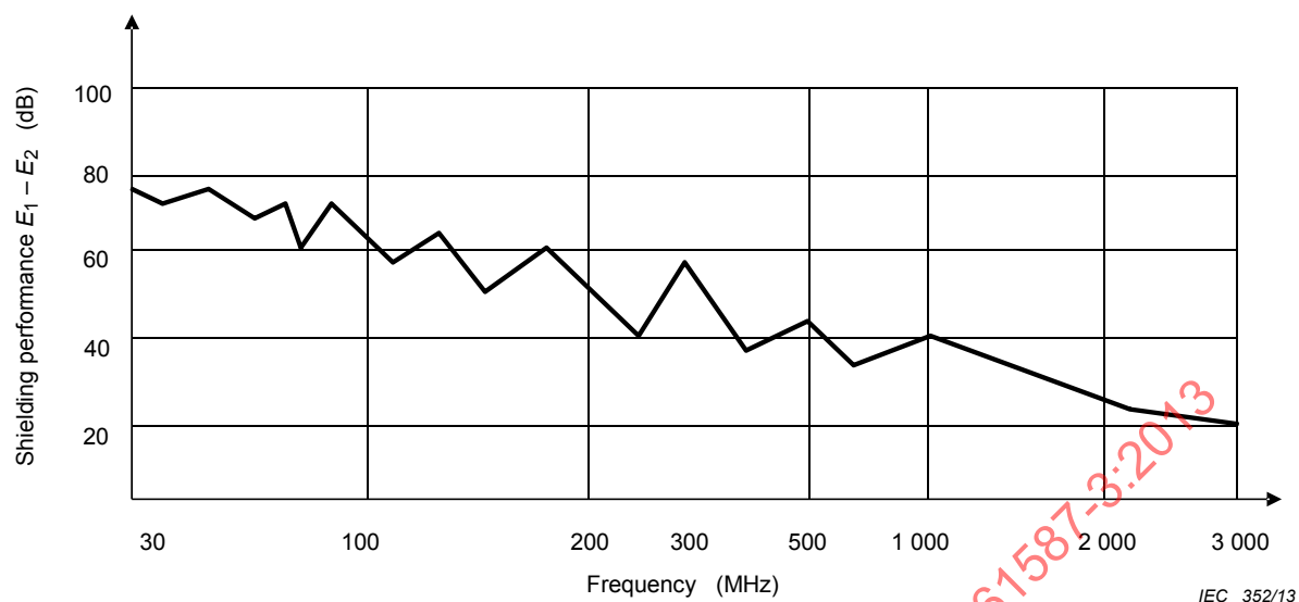
Figure 2 – Example of a measurement data presentation
