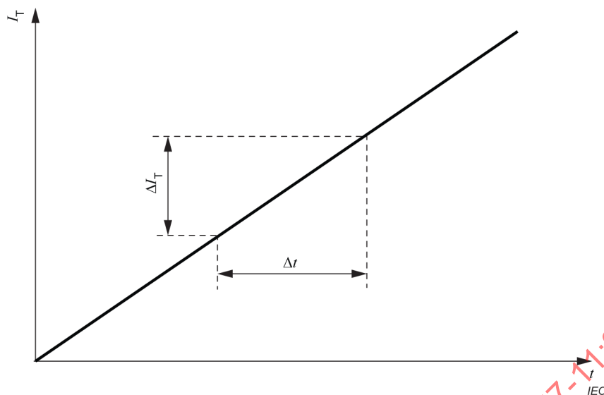
Figure 2 – Maximum gradient of linearly increasing smooth direct test current ( I_T )
