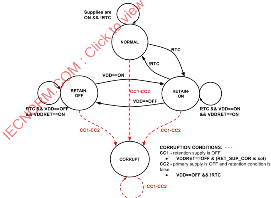
Figure 7—Retention state transition diagram for master/slave-alive style retention
