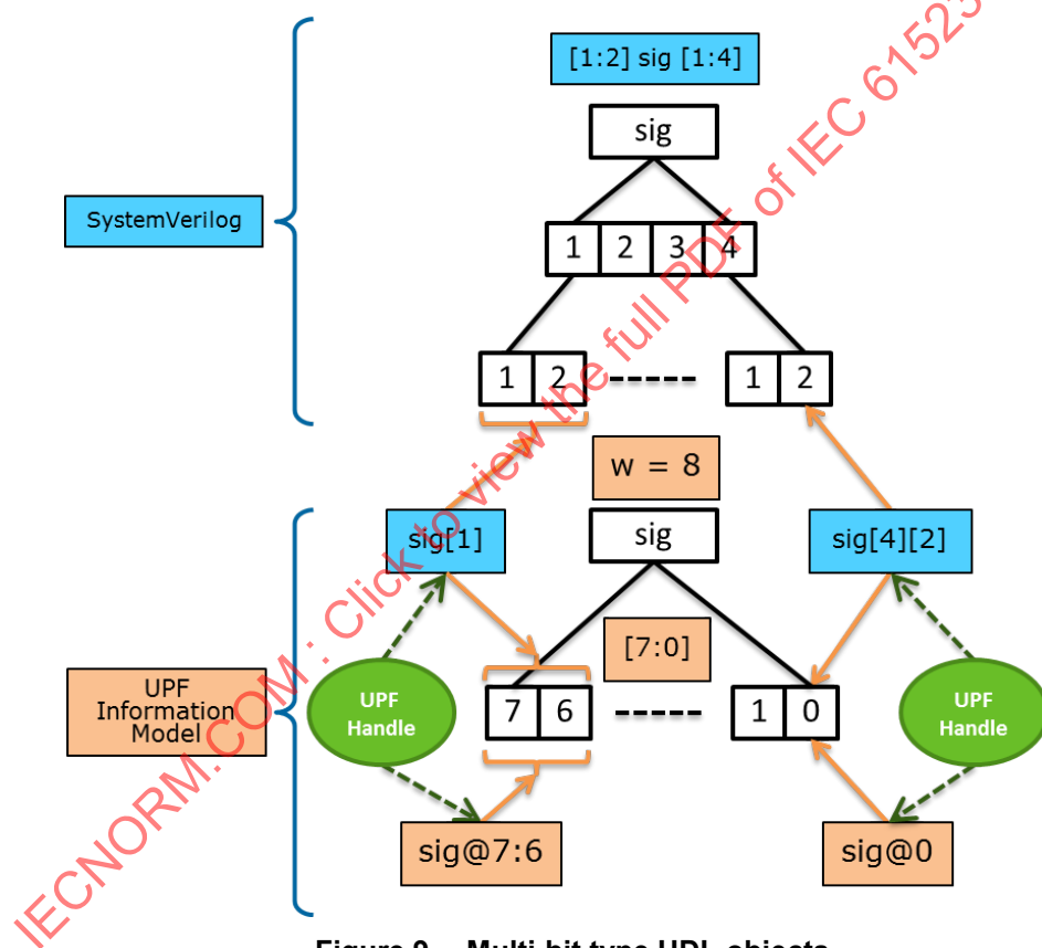
Figure 9 —Multi-bit type HDL objects
