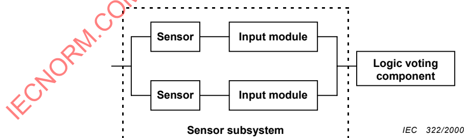
Figure B.2 – Example configuration for two sensor channels
