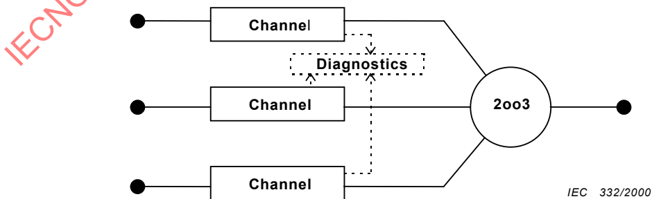
Figure B.12 – 2oo3 physical block diagram
