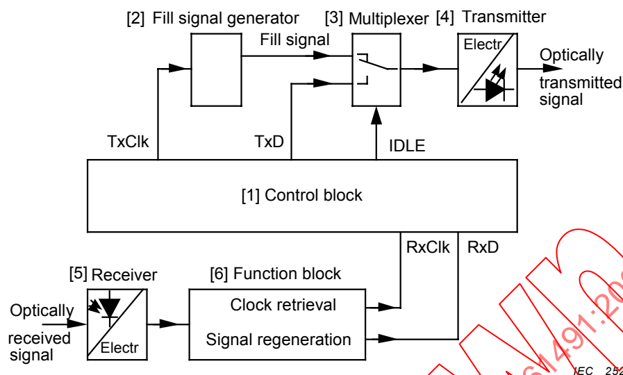
Figure 16 – Functions of a master connection
