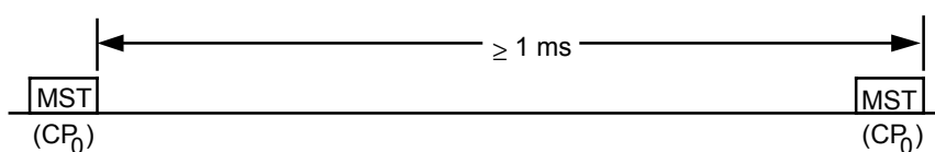
Figure 59 – Timing diagram for CP 0
