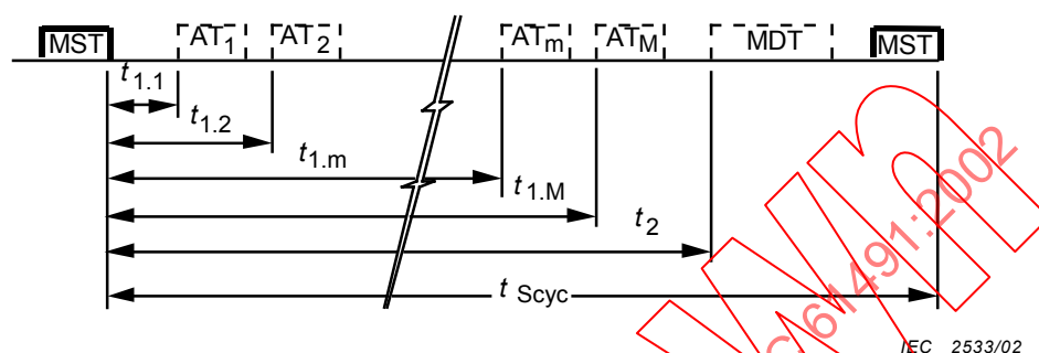
Figure 21 – Access to the transfer medium
