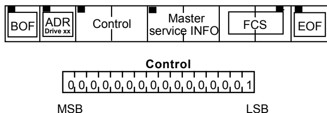
Figure 60 – Structure of the ID request telegram
