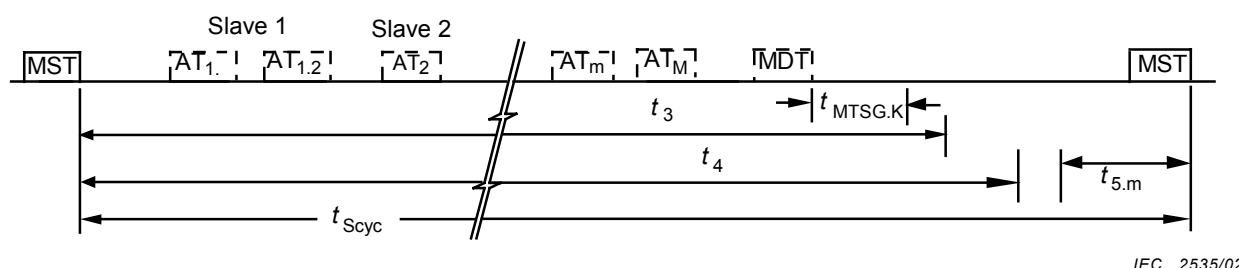
Figure 23 – Validity of command values and feedback acquisition time in the drives
