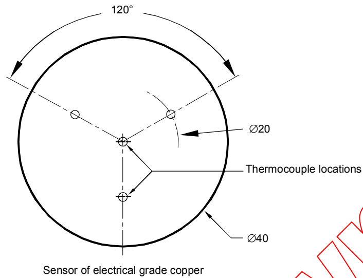
Figure 7a – Installation of thermocouples in the calorimeter
