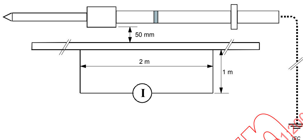
Figure 3a – General arrangement with parallel position
