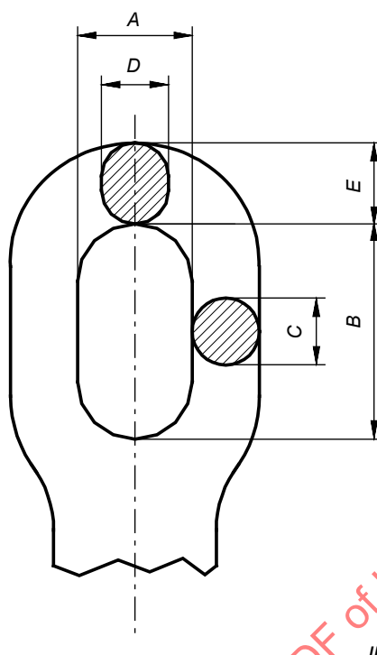
Figure D.1 – Dimensions of eye couplings
