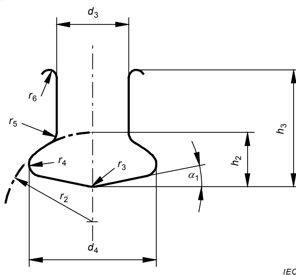
Figure A.2 – Dimensions of GO gauges for ball couplings
