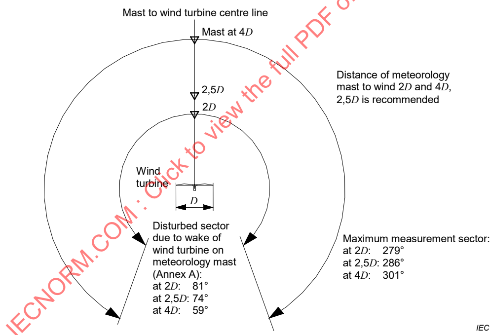
Figure 1 – Requirements as to distance of the wind measurement equipment and maximum allowed measurement sectors
