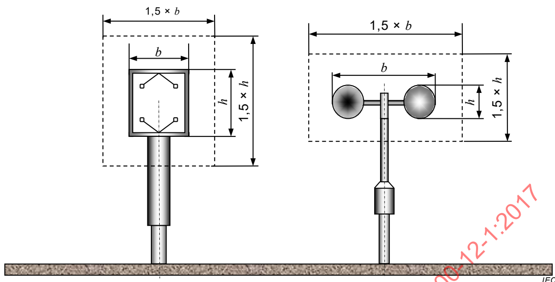
Figure F.1 – Definition of volume for flow uniformity test – The volume will also extend 1,5 \times b in depth (along the flow)
