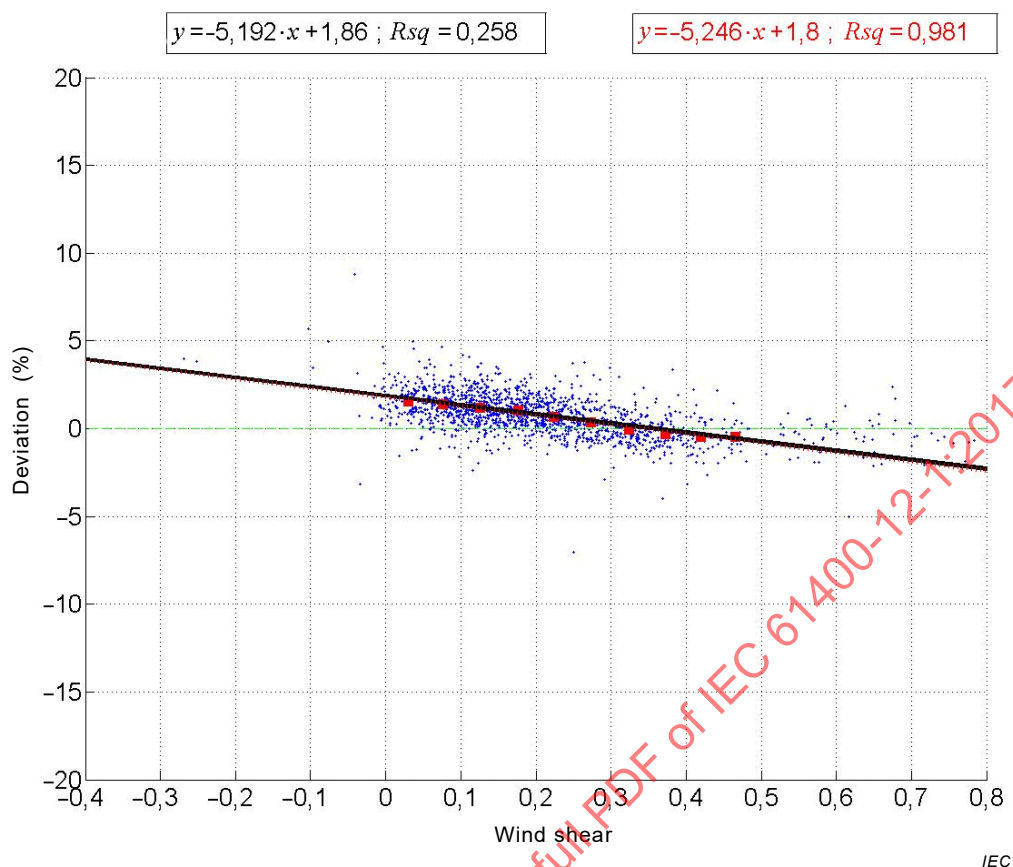
Figure L.2 – Example of sensitivity analysis against wind shear
