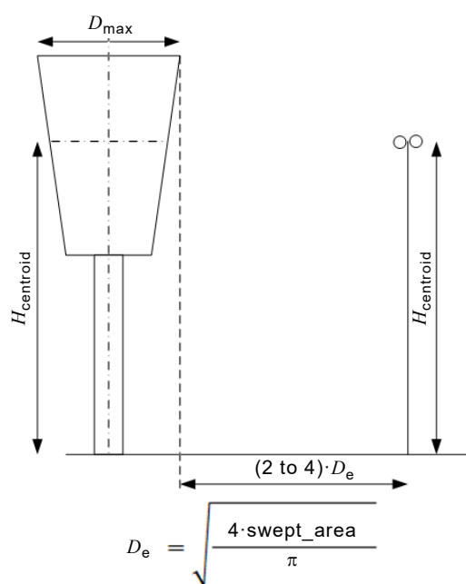
Figure H.1 – Definition of hub height and meteorological mast location for vertical axis wind turbines
