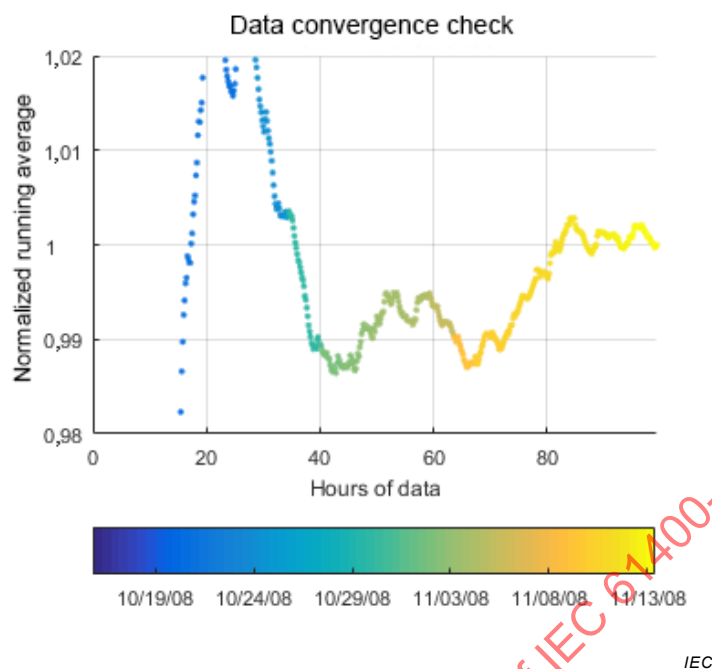
Figure C.18 – Convergence check for 270° bin
