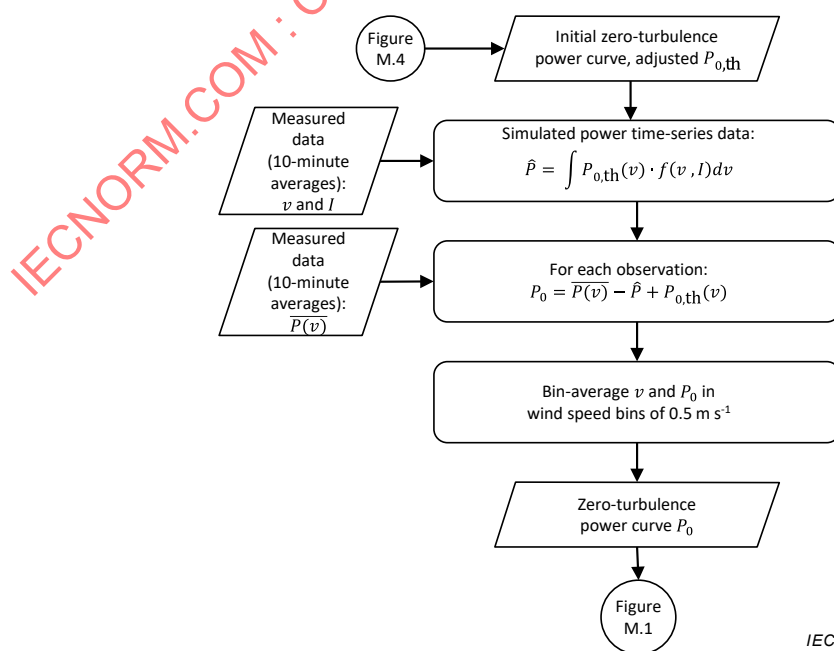
Figure M.6 – Process for obtaining the final zero-turbulence power curve from the measured data
