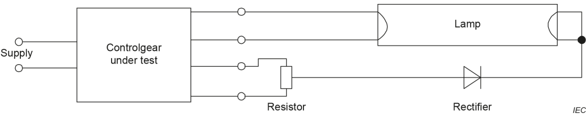
a) Testing the first direction of the rectifying effect
