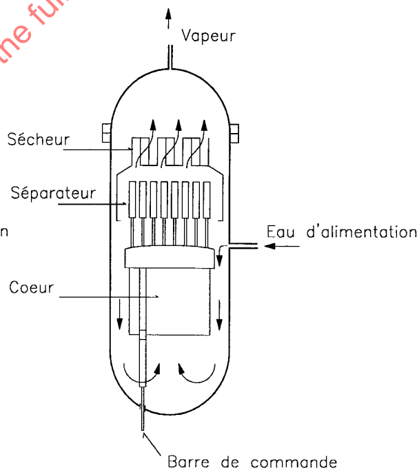
Figure 1d – Circulation naturelle
