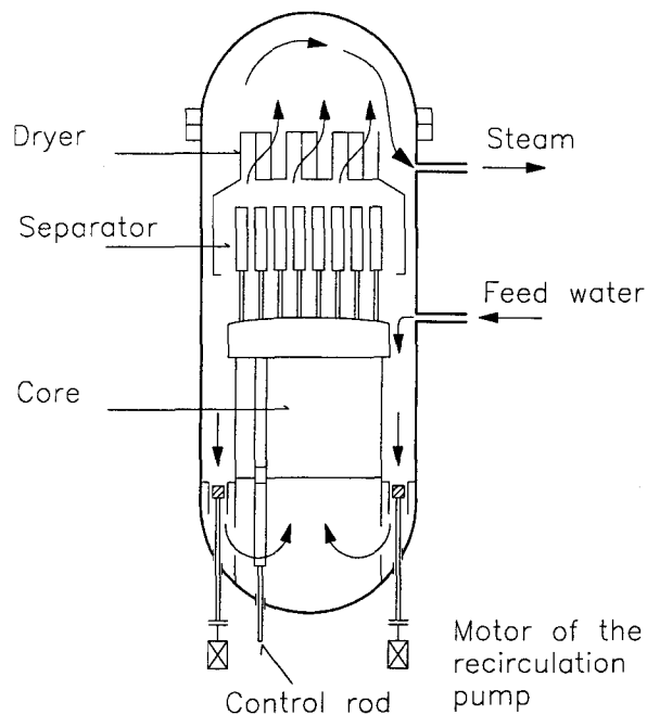
Figure 1a – Internal pumps
