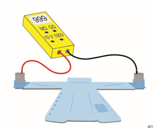
Figure 4 – Test set-up – Resistance point-to-point (cuff-to-cuff procedure)
