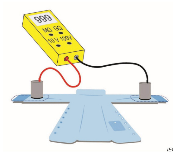
Figure 1 – Test set-up – Resistance point-to-point (sleeve-to-sleeve procedure with insulative sleeve inserts)
