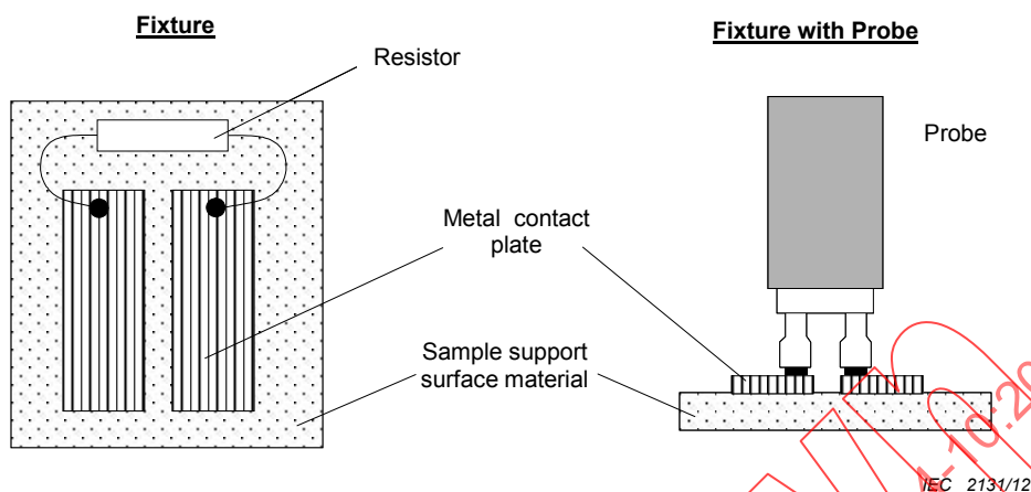
Figure 3 – Resistance verification fixture
