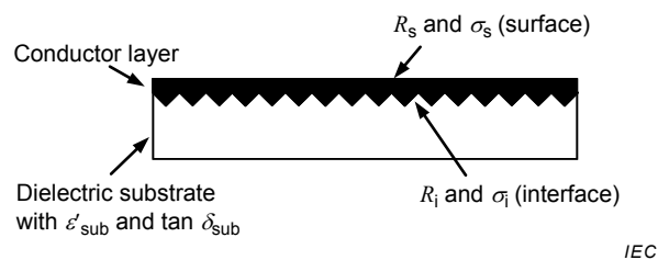
Figure 1 – Surface resistance R_s , surface conductivity \sigma_s , interface resistance R_i , and interface conductivity \sigma_i .
