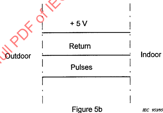
Figure 5 – Antenna position sensor interfaces
