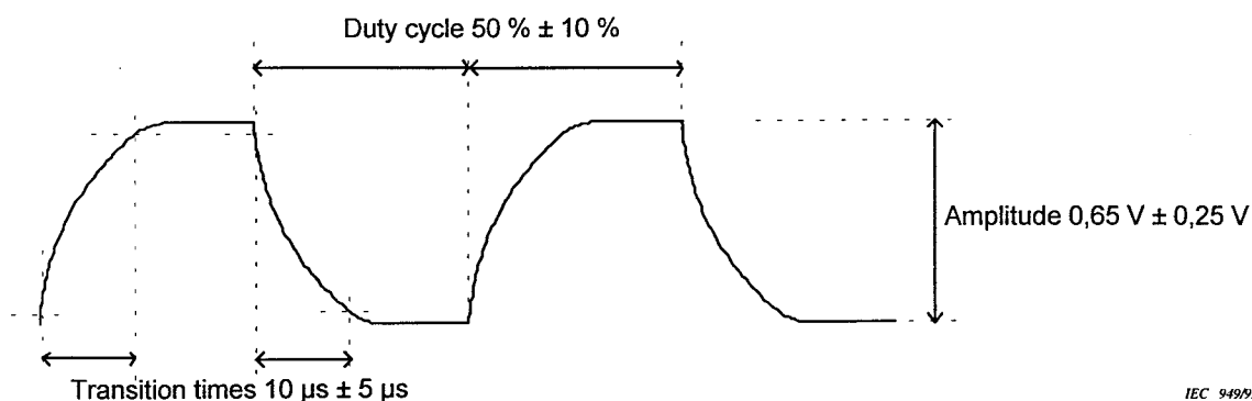
Figure 2 – Control signal for polarswitcher, combined with dual-band block converter, superimposed on supply voltage
