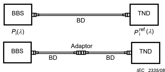
Figure 2a – Attenuation reference measurement
