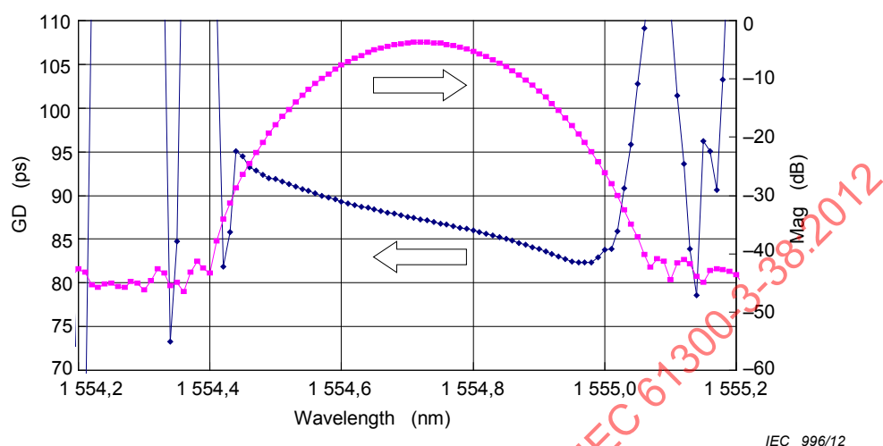
Figure 11 – Measured GD and loss spectra for planar waveguide filter
