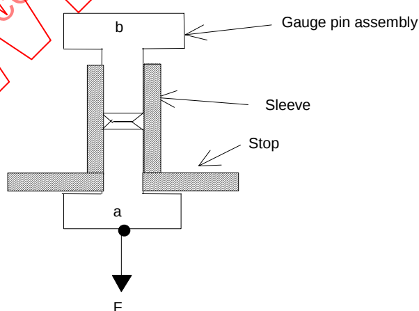
Figure 1 – Test unit with applied force
