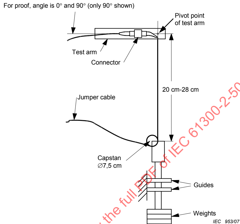
Figure 1 – Proof test apparatus
