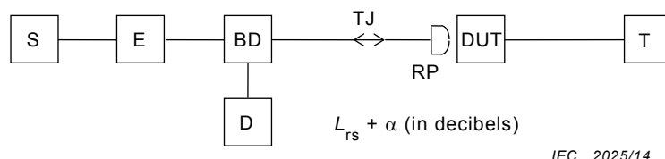
Figure 4 – Measurement set-up for pigtail cord screen testing
