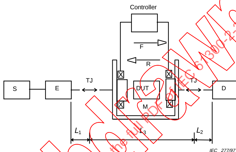
Figure 1 – Measurement set-up
