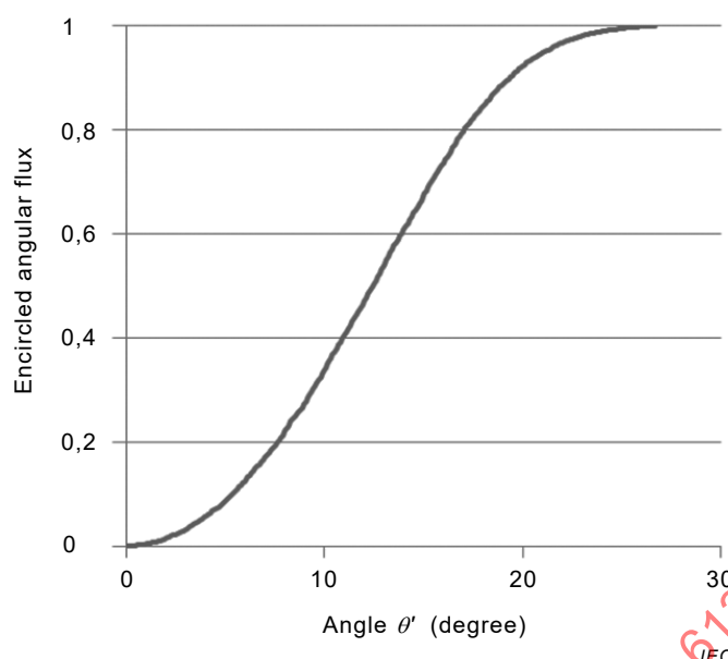
Figure A.2 – Encircled angular flux template example
