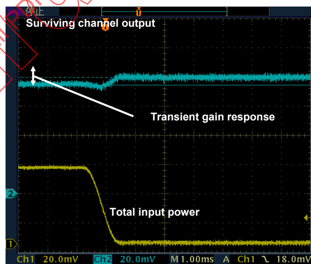
16 dB drop case (rise time = 1 000 µs)
