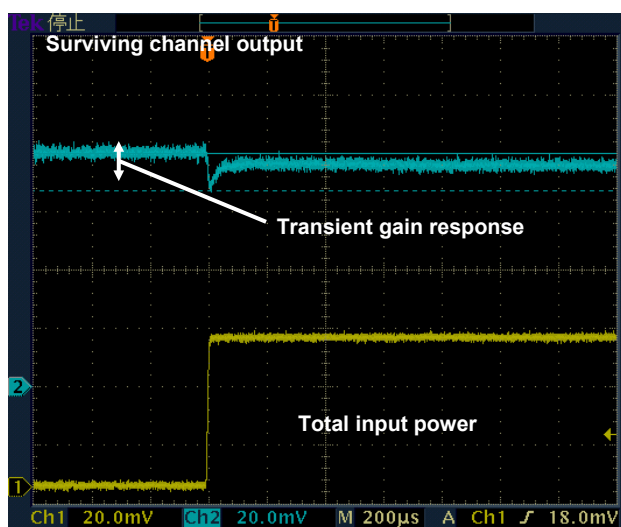
16 dB add case (rise time = 10 µs)
