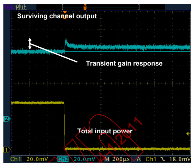
16 dB drop case (rise time = 10 µs)
