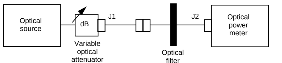
Figure 1a - Input signal power measurement
