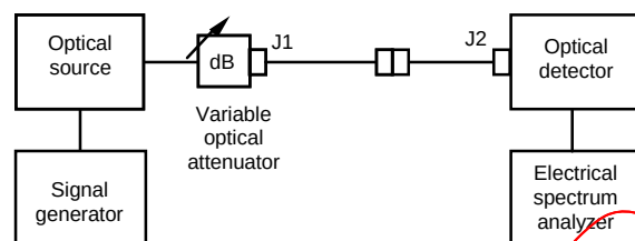
Figure 1b - Measurement of input signal modulated electrical power
