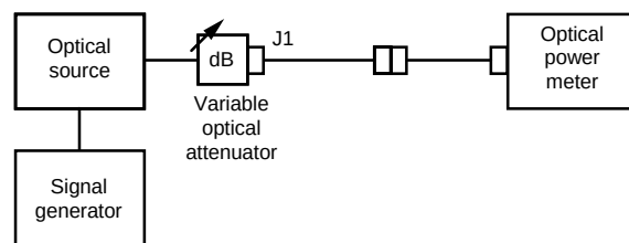
Figure 1a - Measurement of time-averaged input signal optical power
