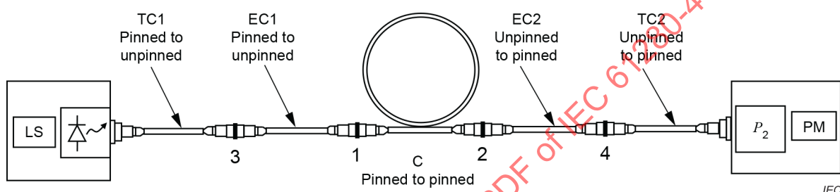
Figure B.7 – Reference measurement for channel test using unpinned power meter
