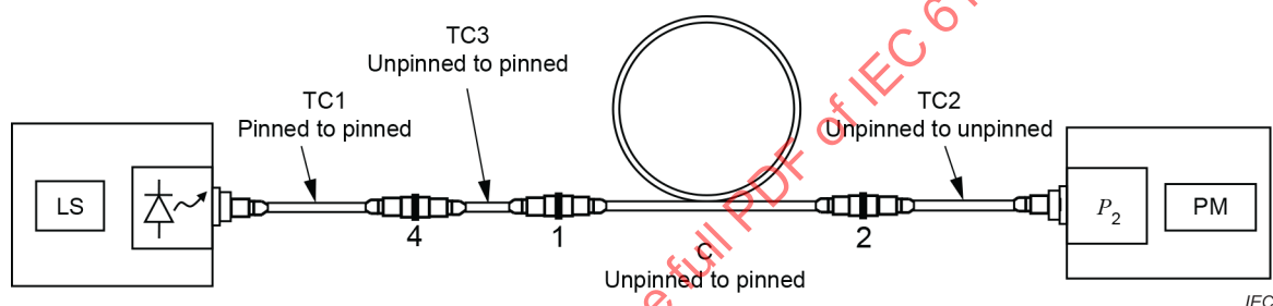
Figure C.3 – Reference measurement for unpinned to pinned cabling using pinned power meter
