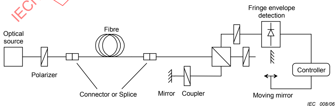
Figure C.2 – Schematic diagram for Method C (TINTY)
