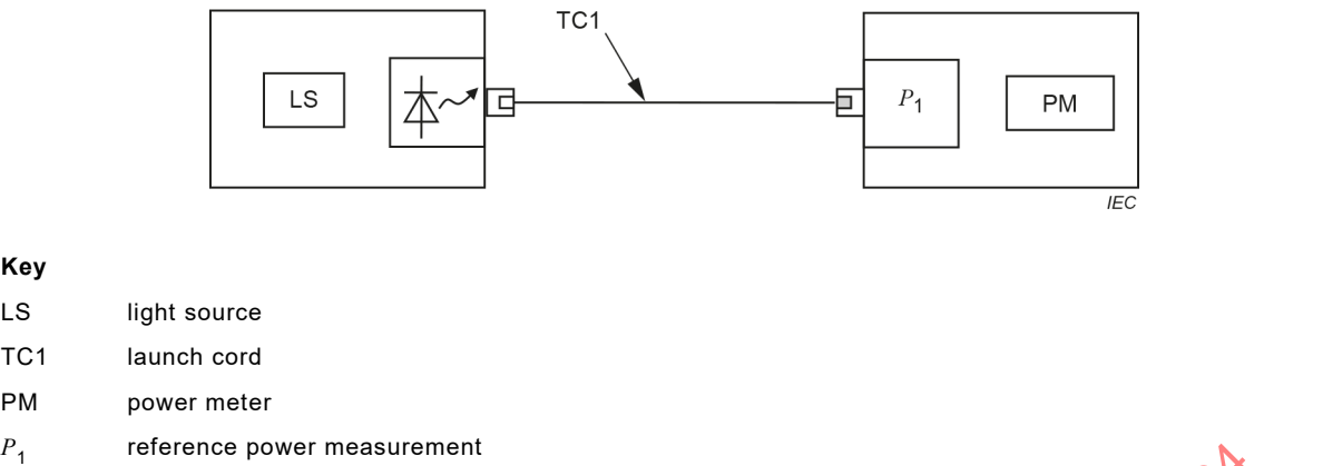
Figure A.1 – One-cord reference measurement
