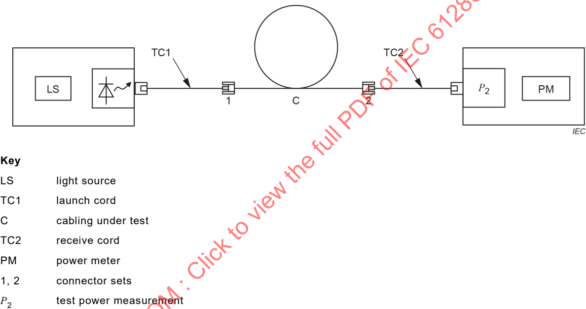
Figure A.2 – One-cord test measurement
