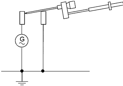
Figure 7c – Circuit arrangement
