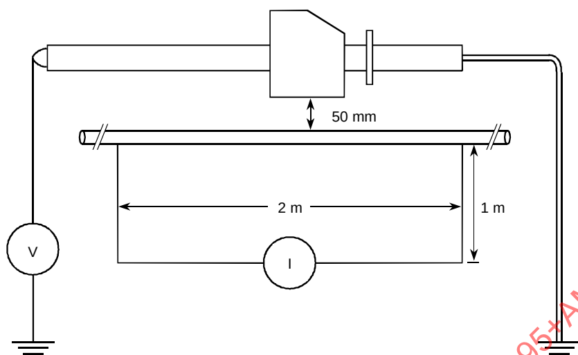
Figure 12a – General arrangement
