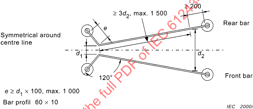
Figure 7b – Dimensions of position bars
