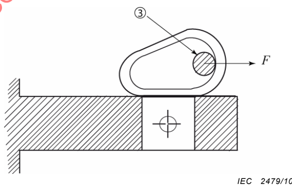
Figure 32b – Bending test
