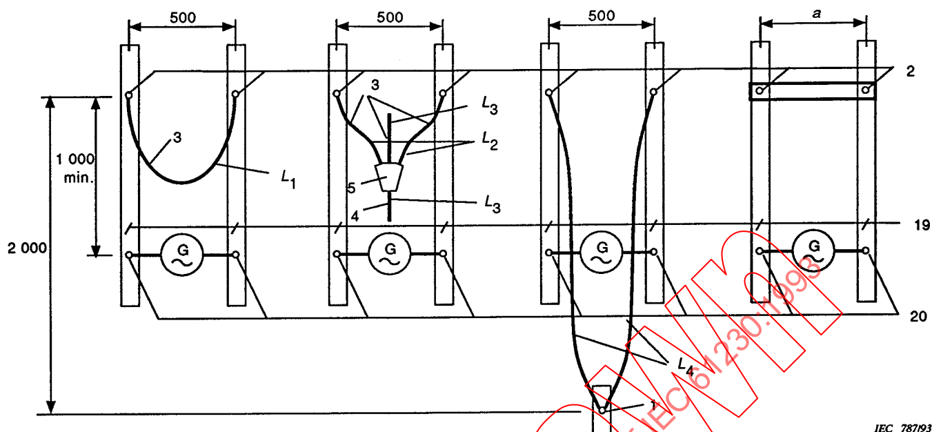
Figure 4d – For testing of bar short-circuiting devices
