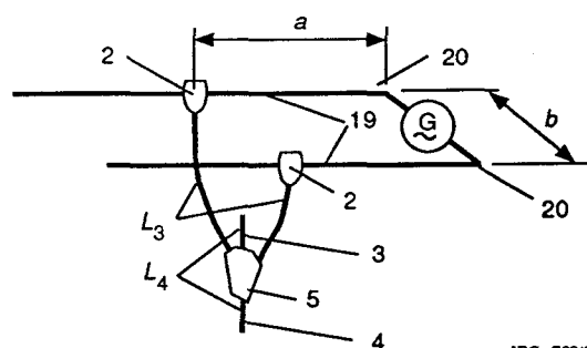
Figure 5b – Test set-up for devices according to figure 2a
