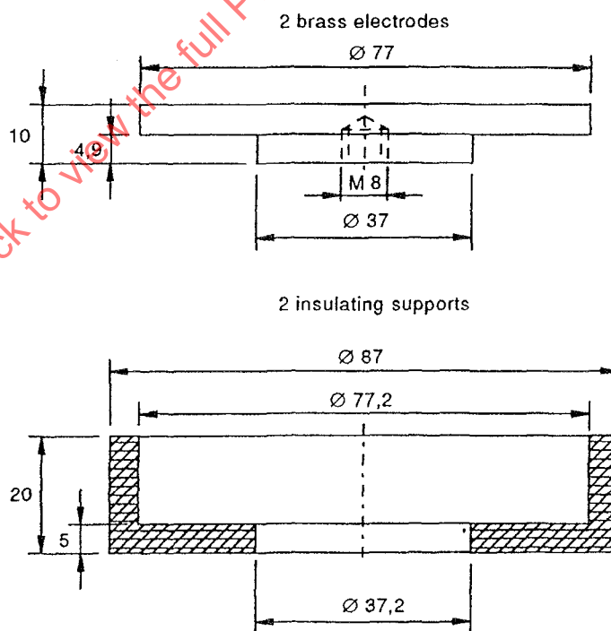
Figure C.3 – Construction drawing for electrode accessories and electrode support
