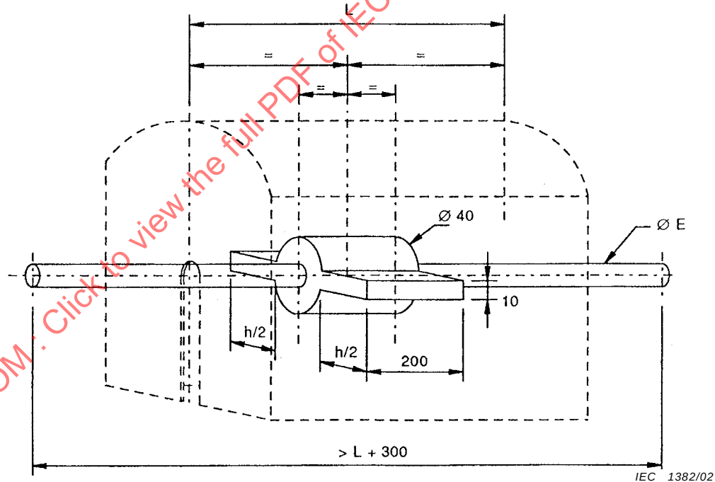
Figure E.3 – Electrode for pin type insulator cover
