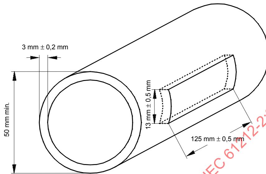
Figure 4a – Test specimen for flammability test cut from tube
