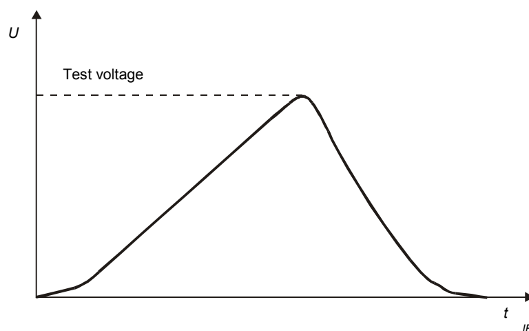
Figure 3 – Example of the applied impulse chopped at the test voltage by flashover of the insulator
