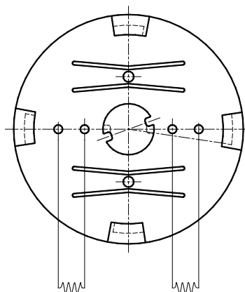
Culot 2G8
