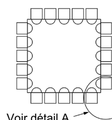
Figure 33 – Porte-puce sans sorties – Cible
