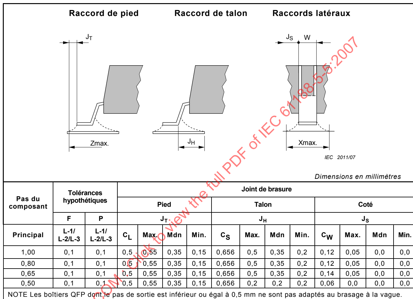
Figure 7 – Conception des raccords de joint de brasure
