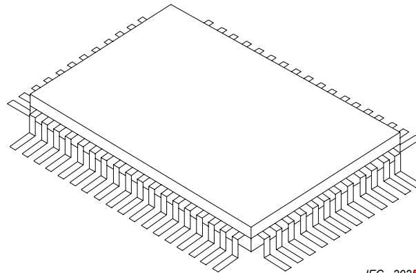
Figure 13 – PLQFP (rectangular)
