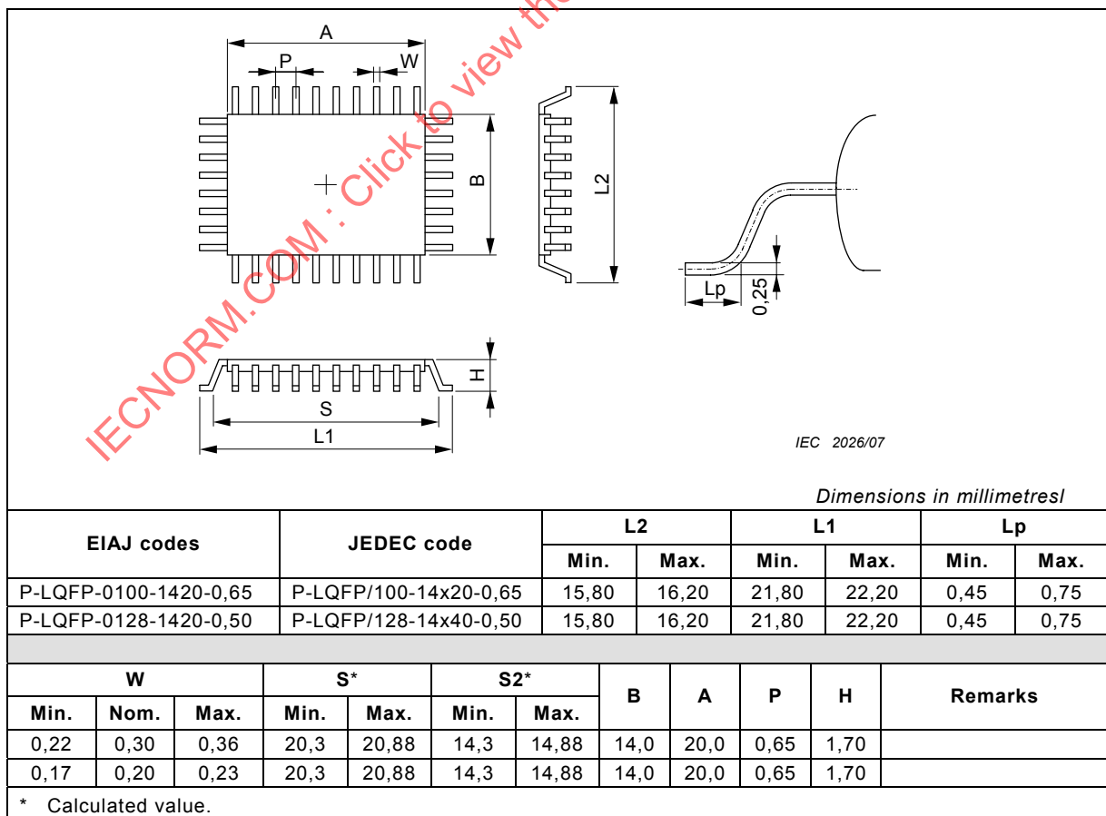
Figure 14 – PLQFP (rectangular) component dimensions
