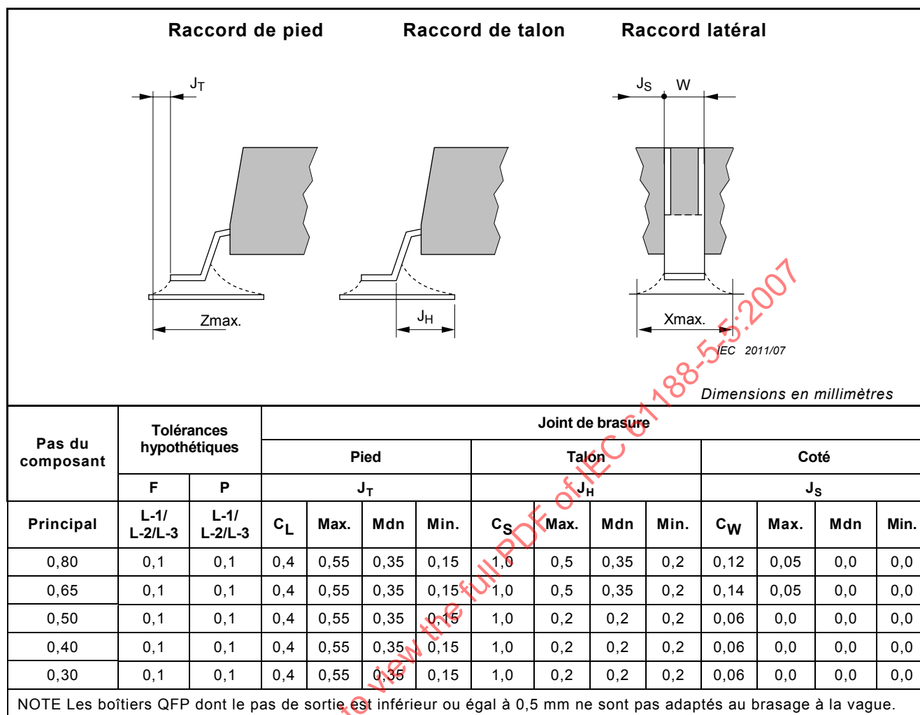
Figure 11 – Conception des raccords de joint de brasure
