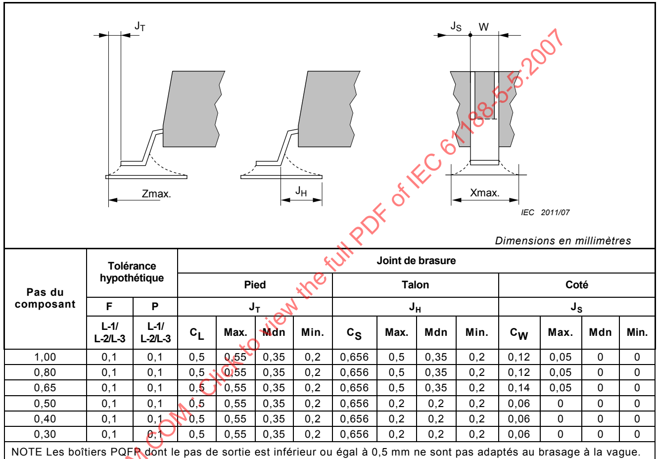
Figure 3 – Conception des raccords de joint de brasure
