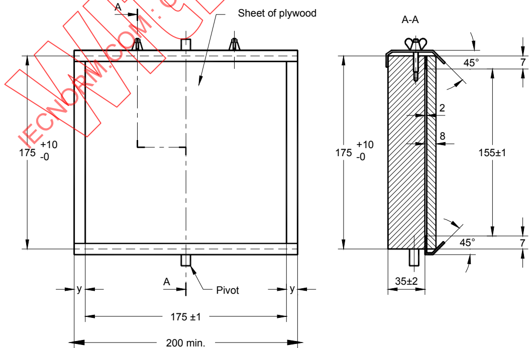
Figure 16 – Mounting support
