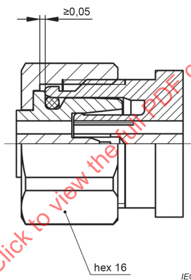
Figure 3 – Screw type connector
