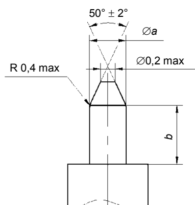
Figure 3 – Gauge pins for socket-centre contact (for dimensions and notes, see Table 3)
