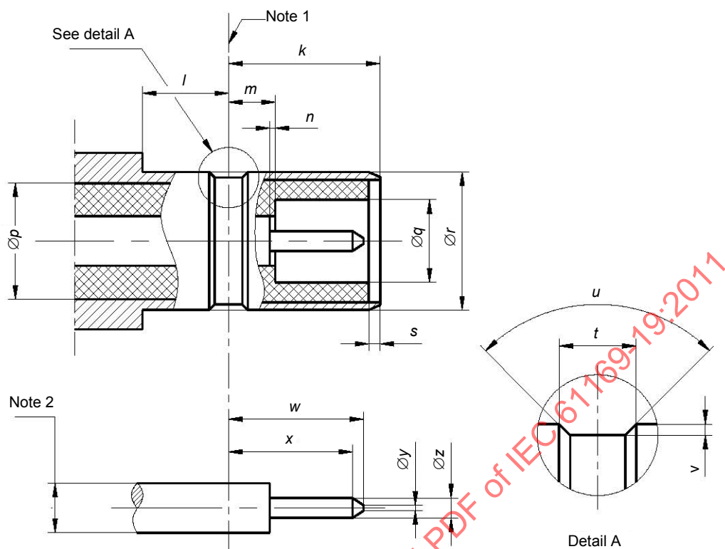
Figure 2 – Connector with pin-centre contact (for dimensions and notes, see Table 2)
