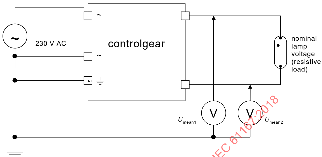
Figure G.3 – Example of a measurement circuit of lamp potential against earth
