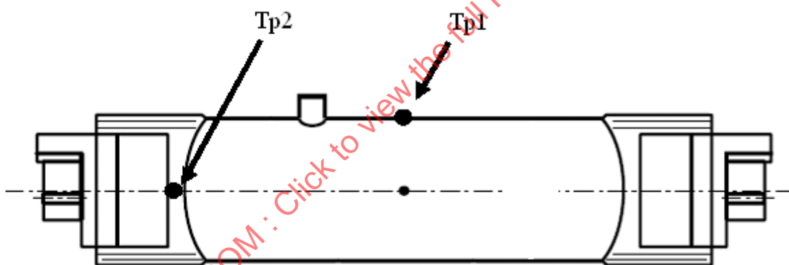
Figure K.9 – Burning position and thermocouple junction fixing points for temperature readings – RX7s and RX7s-24 cap
