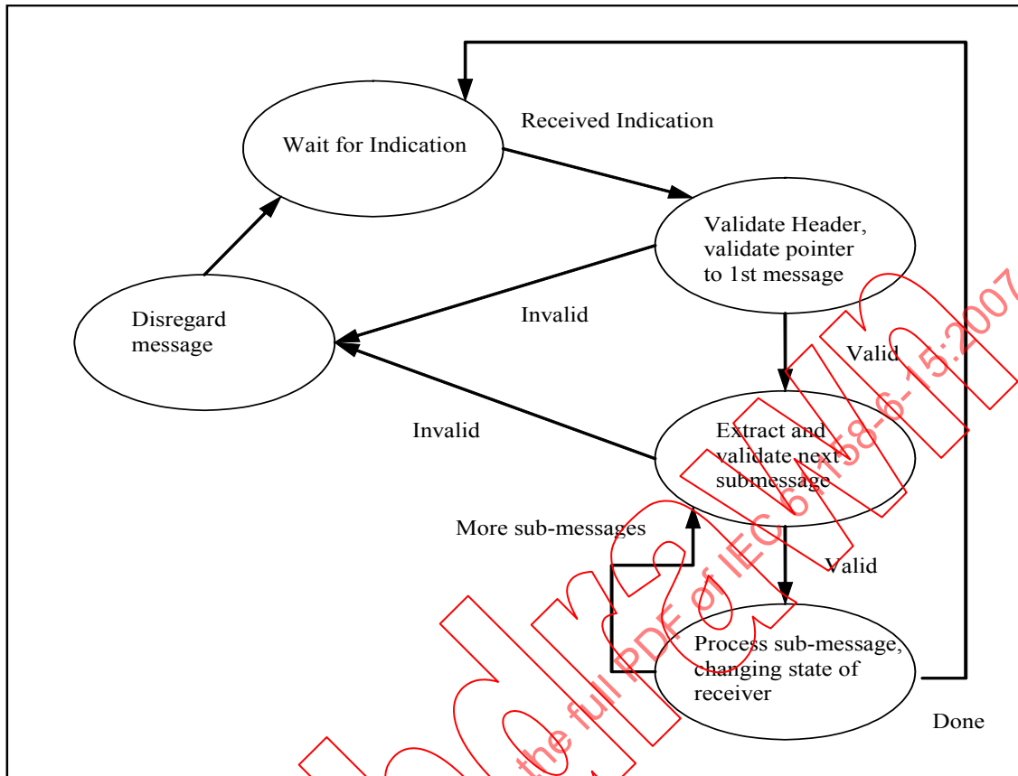
Figure 15 – Publish/subscribe receiver
