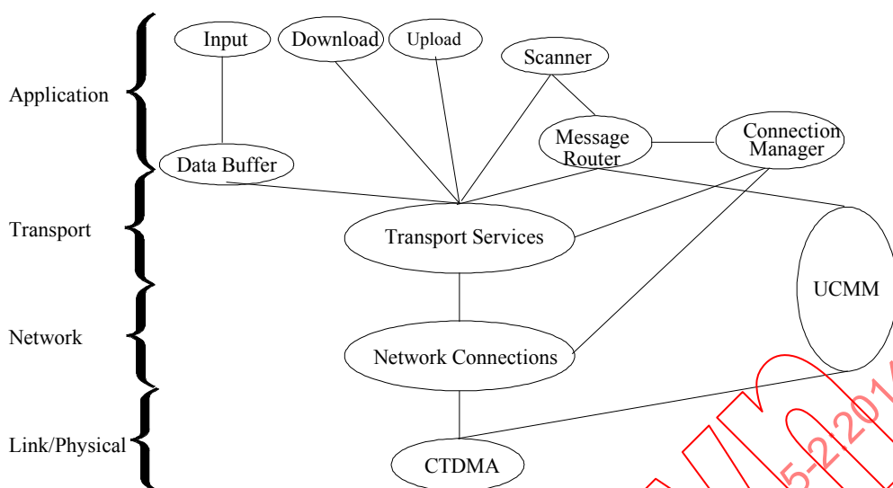
Figure 20 – Context of transport services within the connection model
