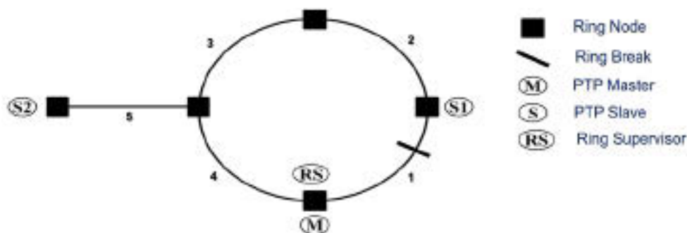
Figure 10 – Path Reconfiguration in a ring topology
