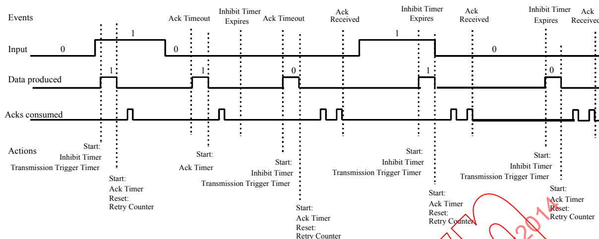
Figure 7 – Example of a COS system with two acking devices
