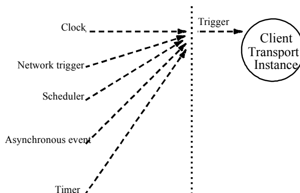
Figure 24 – Triggers
