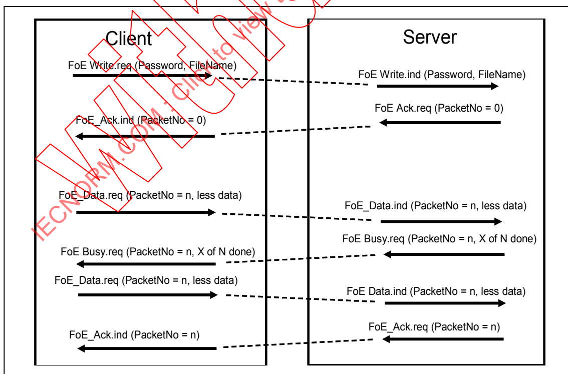
Figure 31 – FoE write sequence with busy
