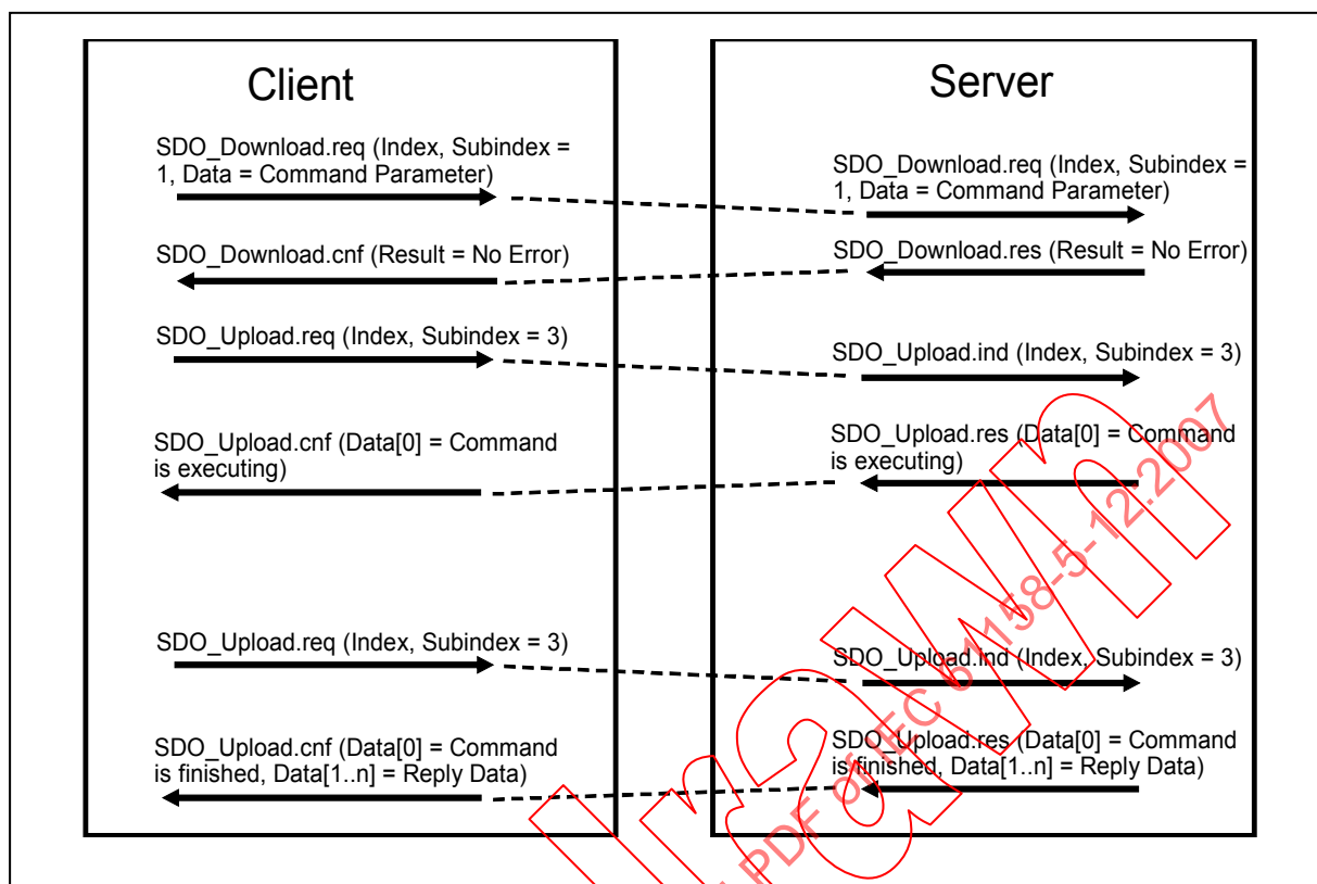
Figure 19 – Command sequence
