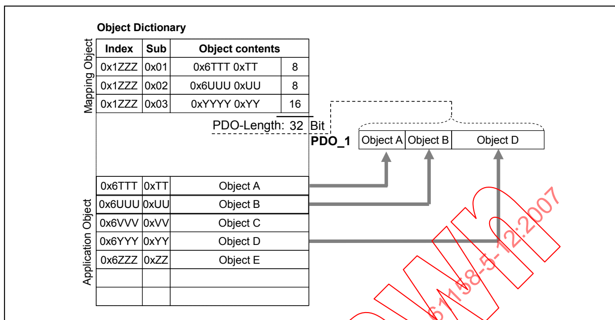
Figure 20 – PDO mapping
