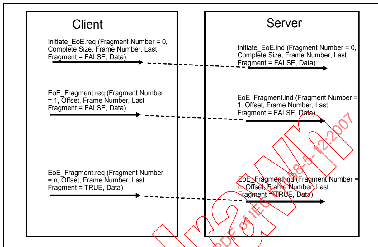
Figure 26 – EoE sequence
