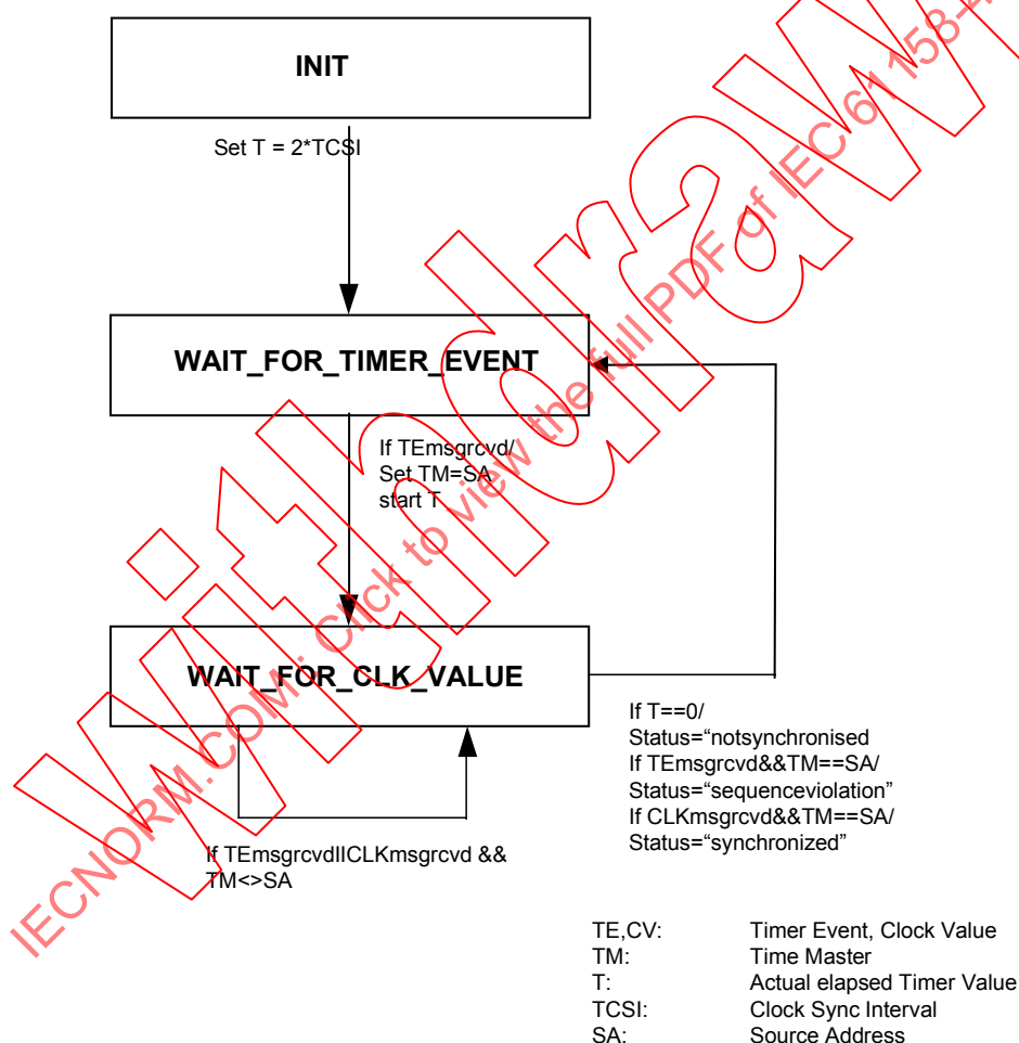
Figure 41 – Time receiver state machine
