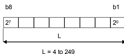
Figure 15 – Length octet coding
